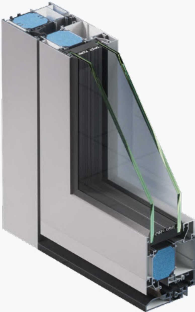
TLS 80 Hybrid Section
